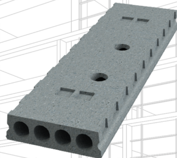
Carottages (10 cm, 12 cm, 15 cm, 20 cm)
